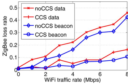
Fig. 14. ZigBee packet-loss rate in TDMA mode.
