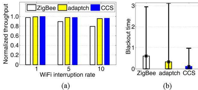
Fig. 18. Performance of CCS versus ideal adaptive channel allocation ( adaptch ). (a) Normalized throughput (ratio of the number of uniquely received packets to those sent). (b) Blackout time (the number of consecutive superframes with beacon losses) when WiFi interrupts 10 times in 10 min. Error bars show the maximum and minimum values.
