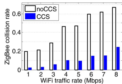
Fig. 12. Packet-loss rate under asymmetric interference.
