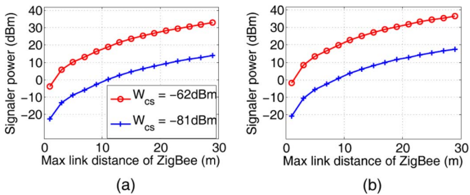
Fig. 10. Required signaling power to ensure the WPAN is sensible by WiFi: (a) uplink; (b) downlink.
