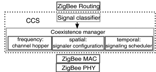
Fig. 7. Architecture of the CCS framework.
