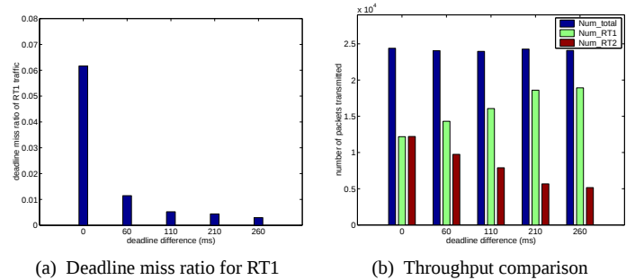
Fig. 11. More experimental results for RT traffic with an EDF queue
