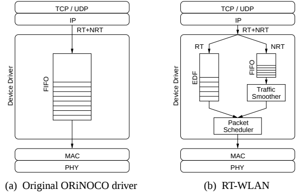
Fig. 4. Comparison of two device driver architectures
