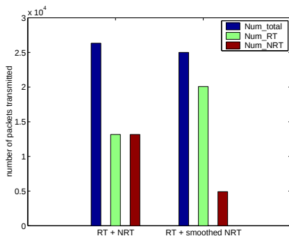
Fig. 13. Throughput comparison for adaptive traffic smoothing
