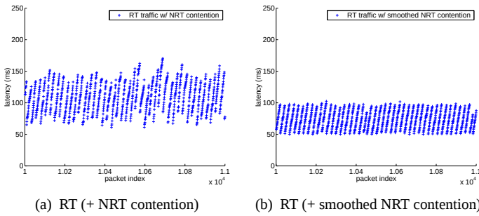
Fig. 12. Latency comparison for adaptive traffic smoothing
