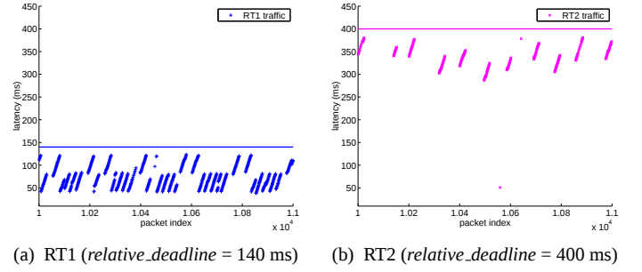
Fig. 10. Latency comparison for RT traffic with an EDF queue
