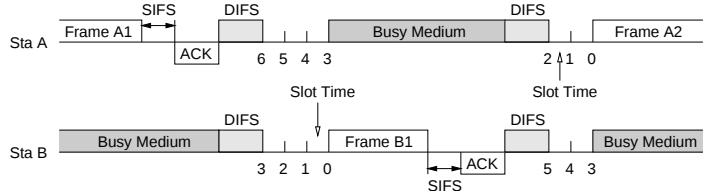
Fig. 3. An example of data frame transmissions and backoff decrements
