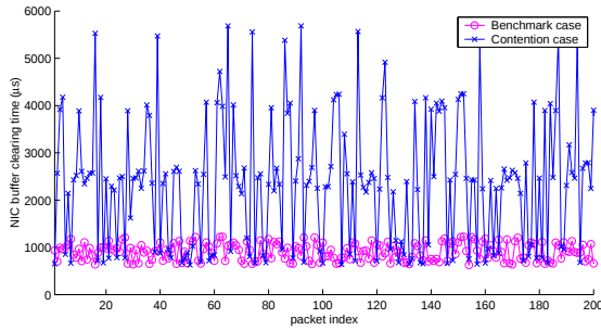
Fig. 6. Comparison of NIC buffer clearing time
