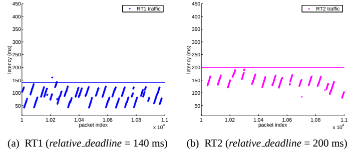
Fig. 9. Latency comparison for RT traffic with an EDF queue
